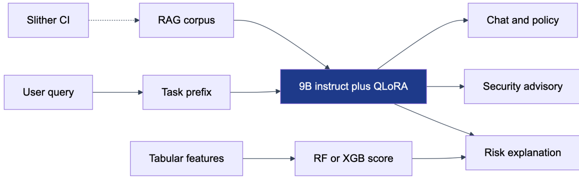
Figure 4.2: Unified fine-tuned 9B assistant with RAG, tabular risk scoring, and static-analysis guardrails (design).
