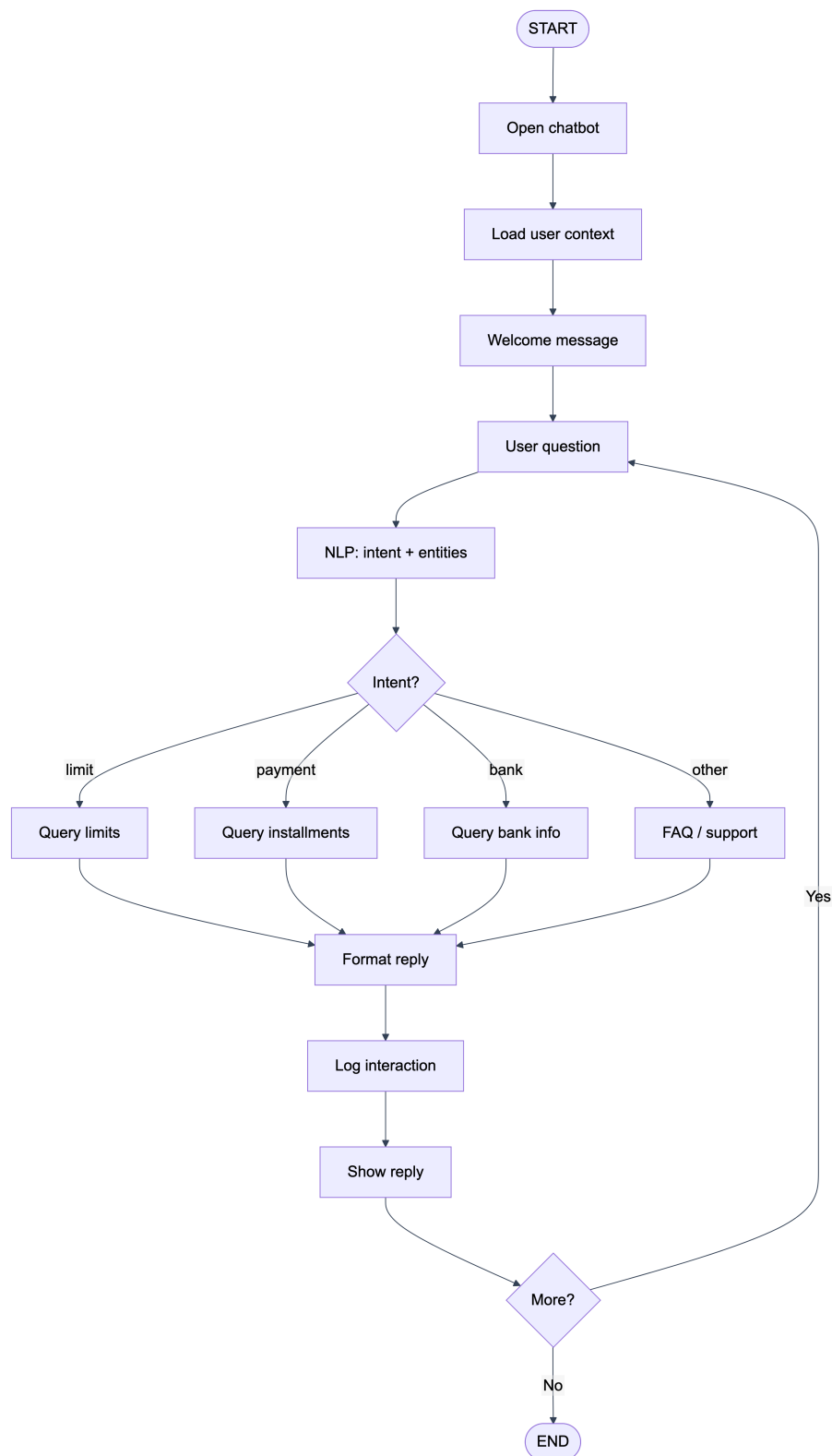
Figure 3.11: Activity Diagram AI Chatbot Interaction Flow
