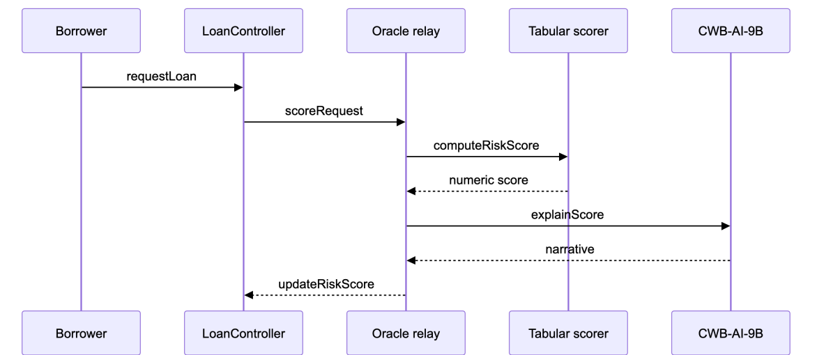
Figure 4.5: Oracle-mediated loan workflow with tabular score and 9B explanation (design).
