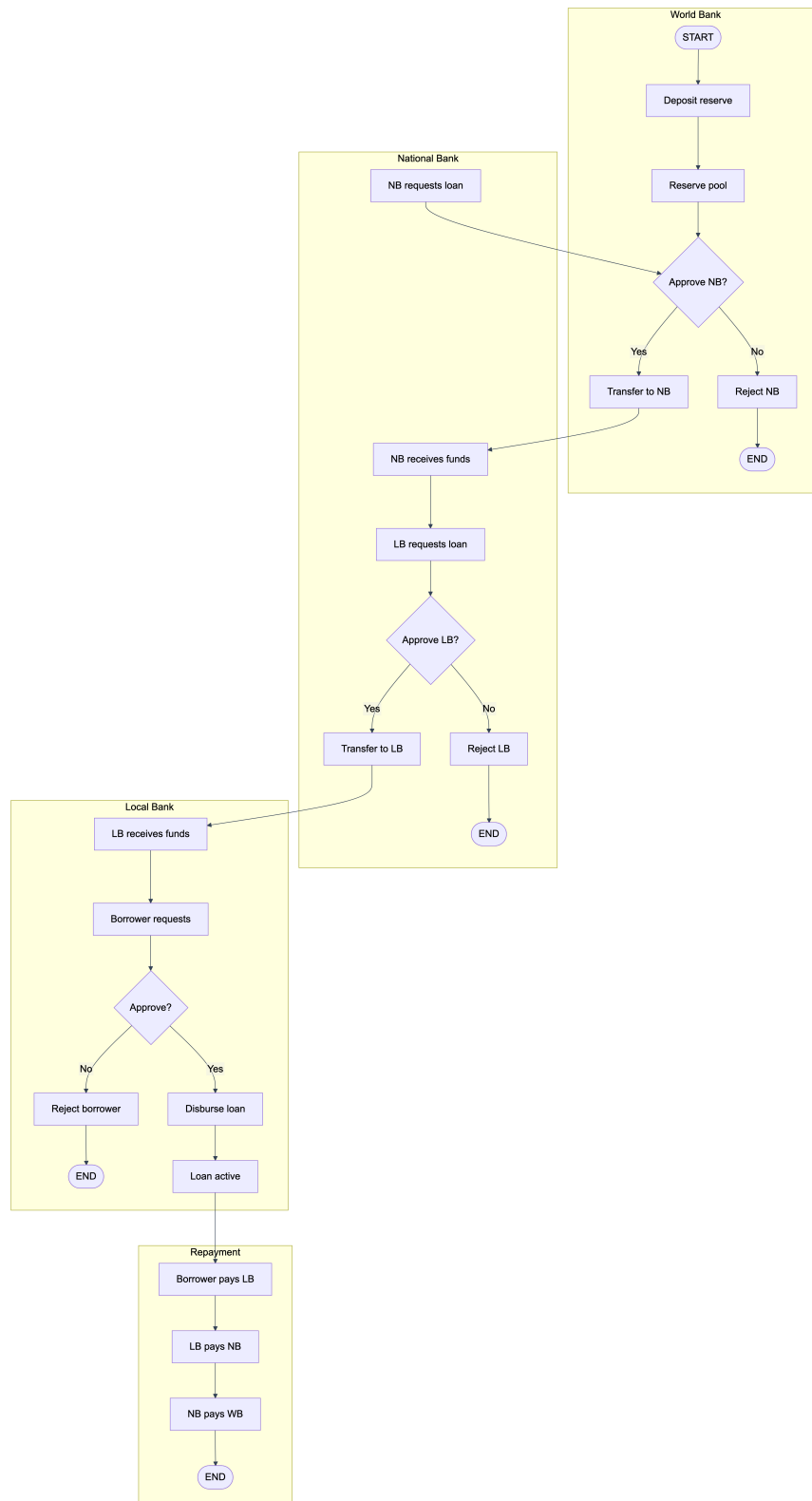
Figure 3.8: Activity diagram illustrating the hierarchical capital flow from the World Bank Reserve through National Bank to Local Bank tiers, including reserve ratio checks and loan disbursement decision points.
