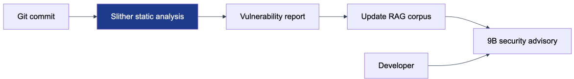
Figure 4.6: Security CI pipeline: static analysis findings inform RAG; 9B provides advisory triage (design).
