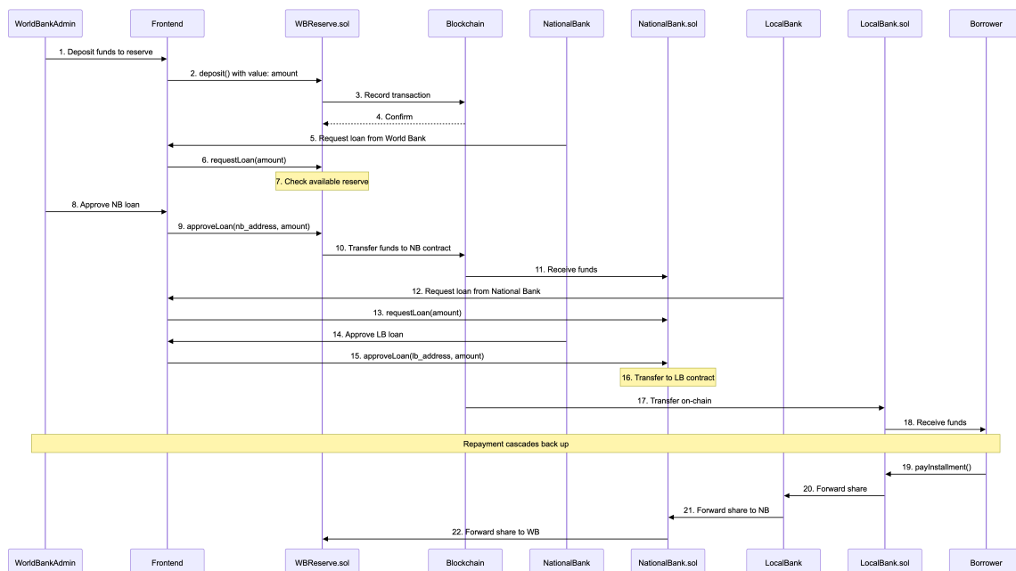
Figure 3.27: Sequence Diagram 6 Hierarchical Banking
