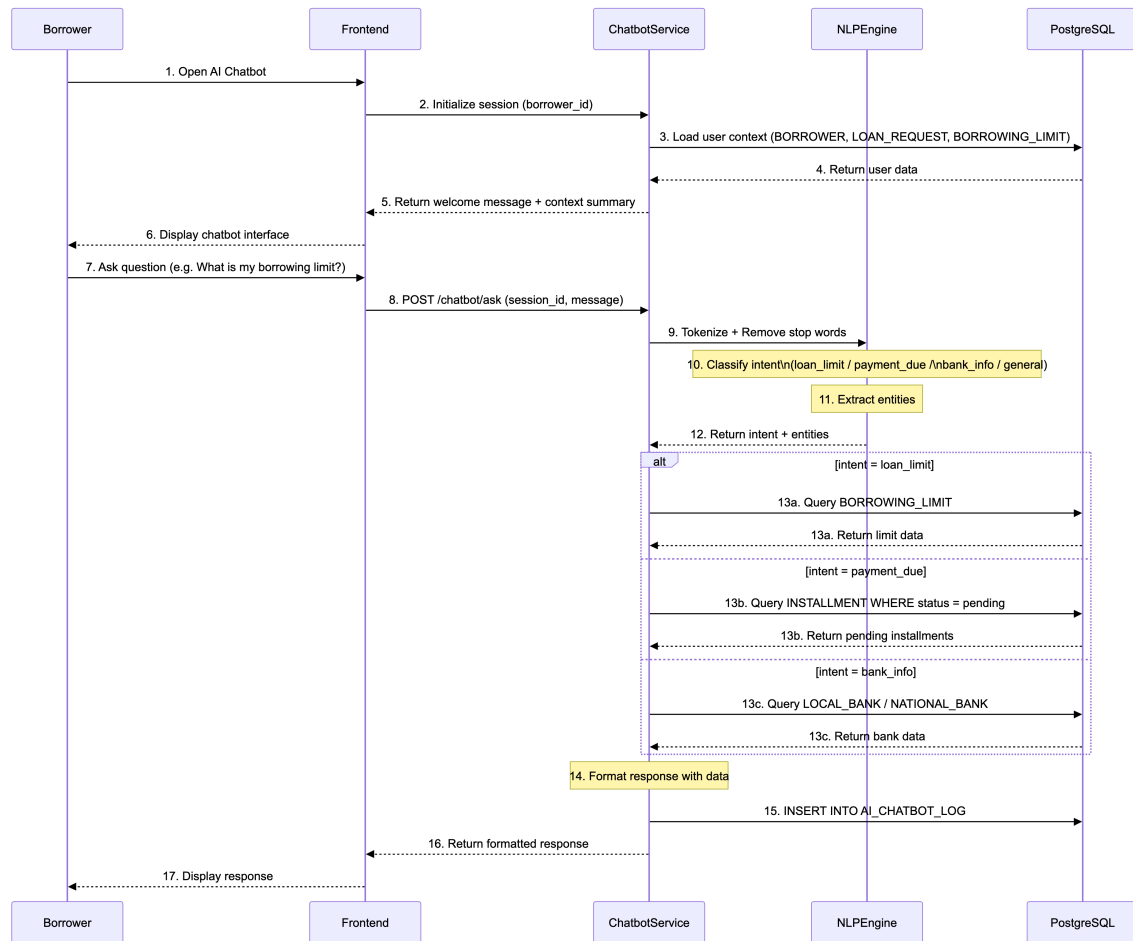
Figure 3.26: Sequence Diagram 5 AI Chatbot Interaction
