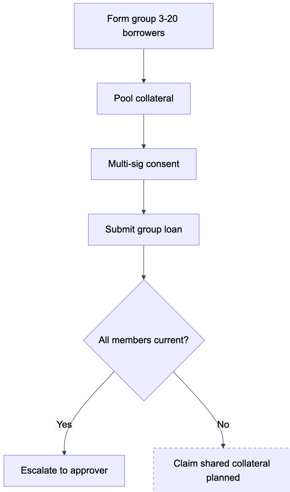
Figure 3.15: Activity diagram: solidarity group formation, consent, disbursement, and mutual liability — «planned» (design).
