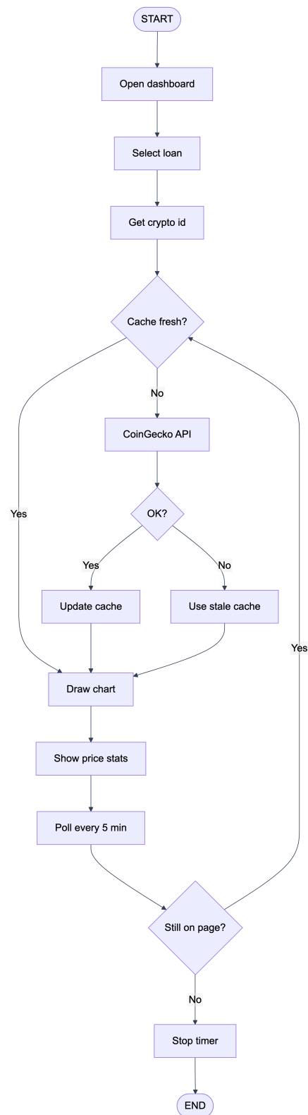
Figure 3.12: Activity diagram showing the market data viewing flow, in which authenticated users fetch live cryptocurrency price feeds via the off-chain API layer before interacting with loan sizing interfaces.
