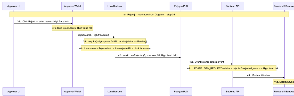
Figure 3.22: Sequence Diagram 1B Reject Path - alt Reject
