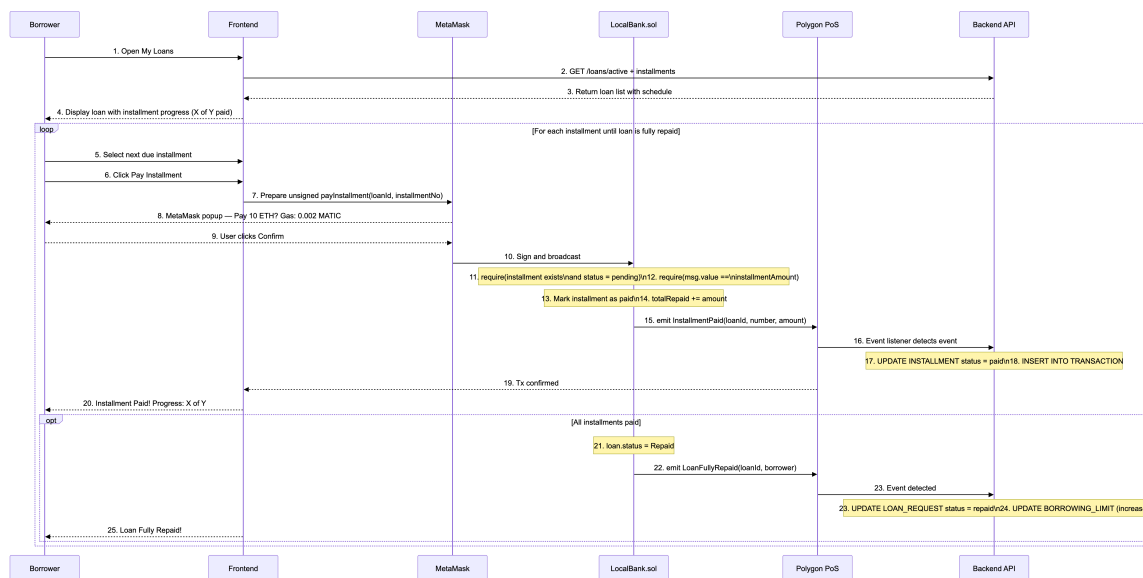
Figure 3.23: Sequence Diagram 2 Installment Payment Loop
