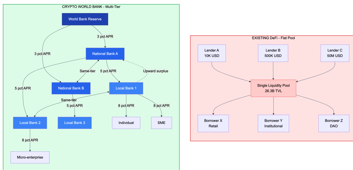
Figure 1.2: Architectural comparison between existing flat-pool DeFi lending protocols and the Crypto World Bank's hierarchical multi-tier model.
