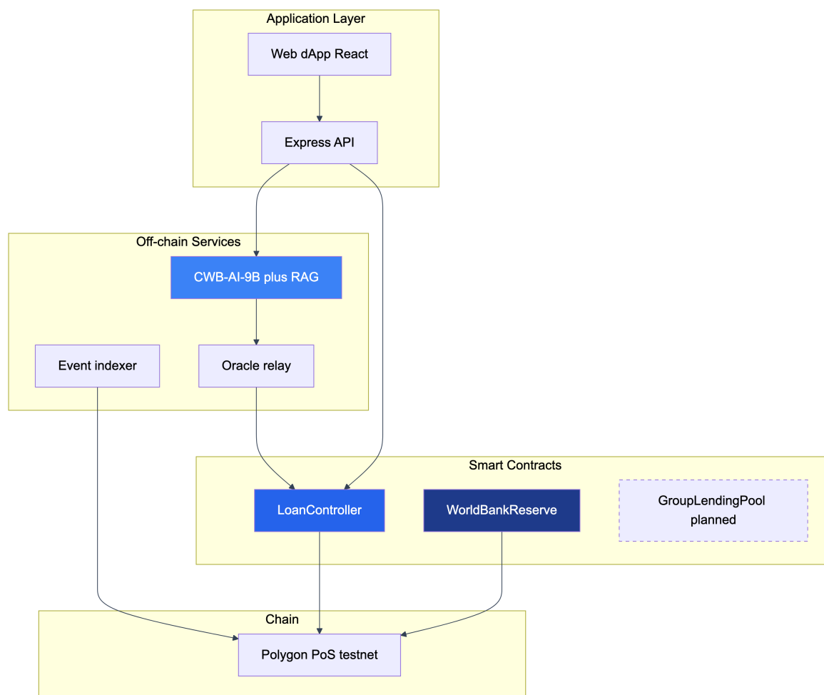
Figure 1.3: Blockchain stack layers connecting the dApp, off-chain services (indexer, oracle, CWB-AI-9B), smart contracts, and Polygon PoS testnet (design).
