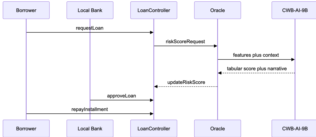
Figure 1.4: Transaction lifecycle for loan request, oracle risk update, approval, and repayment (design).
