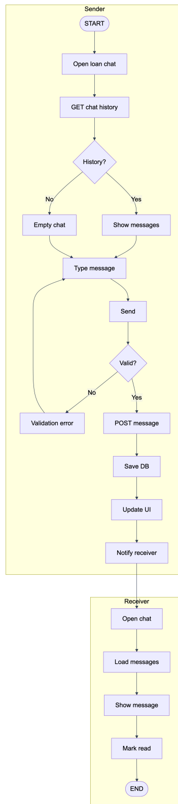
Figure 3.10: Activity Diagram Chat System Flow
