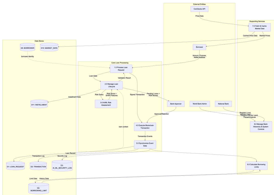
Figure 3.19: Level-1 data flow diagram decomposing the core lending subsystem, showing input/output data flows among borrowers, approvers, the smart contract layer, the PostgreSQL database, and the AI/ML monitoring service.
