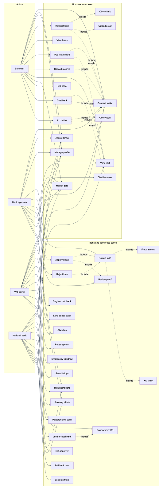
Figure 3.6: Use case diagram for the Crypto World Bank platform, showing interactions among four primary actors (World Bank Admin, National Bank, Local Bank Approver, Borrower) across 29 identified use cases, including registration, loan request, approval workflow, and repayment.
