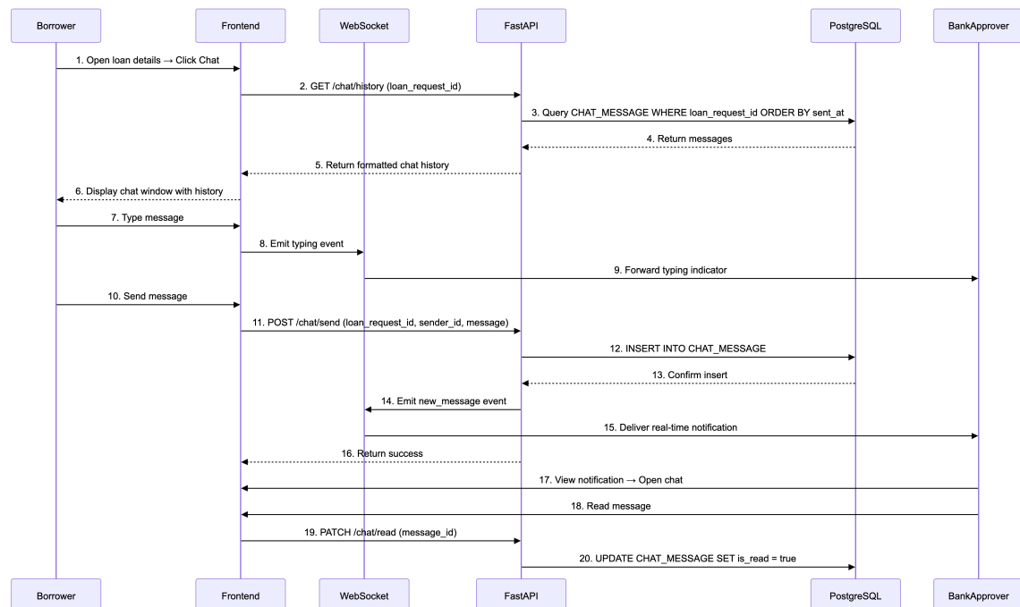
Figure 3.25: Sequence Diagram 4 Chat System
