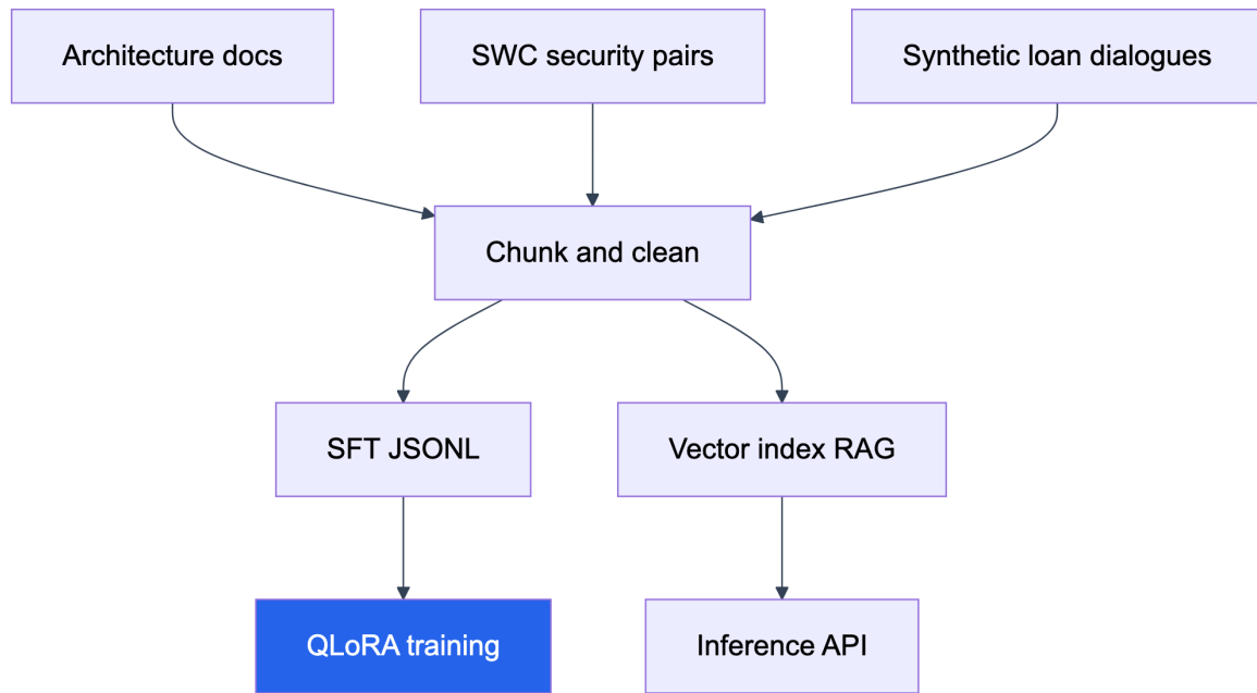
Figure 4.3: Training data pipeline for unified 9B fine-tuning (design).
