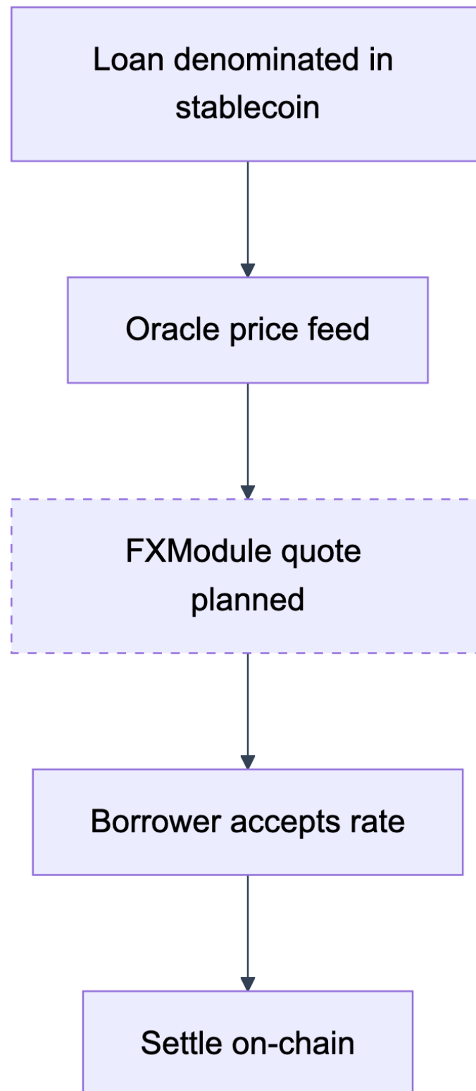
Figure 3.16: Activity diagram: oracle-priced FX conversion for loan denomination — «planned» (design).
