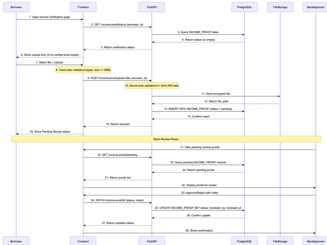
Figure 3.24: Sequence Diagram 3 Income Verification
