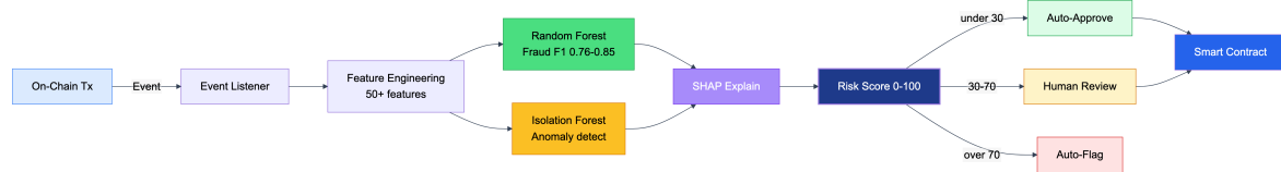
Figure 3.2: AI/ML security analytics pipeline: off-chain model inference integrated with on-chain lending decisions through the risk scoring API.
