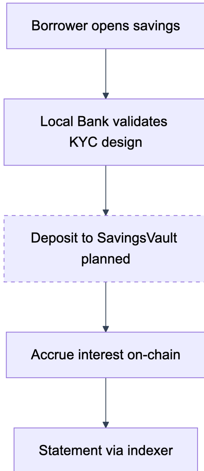
Figure 3.14: Activity diagram: deposit mobilization (savings account opening and accrual) — «planned» (design).
