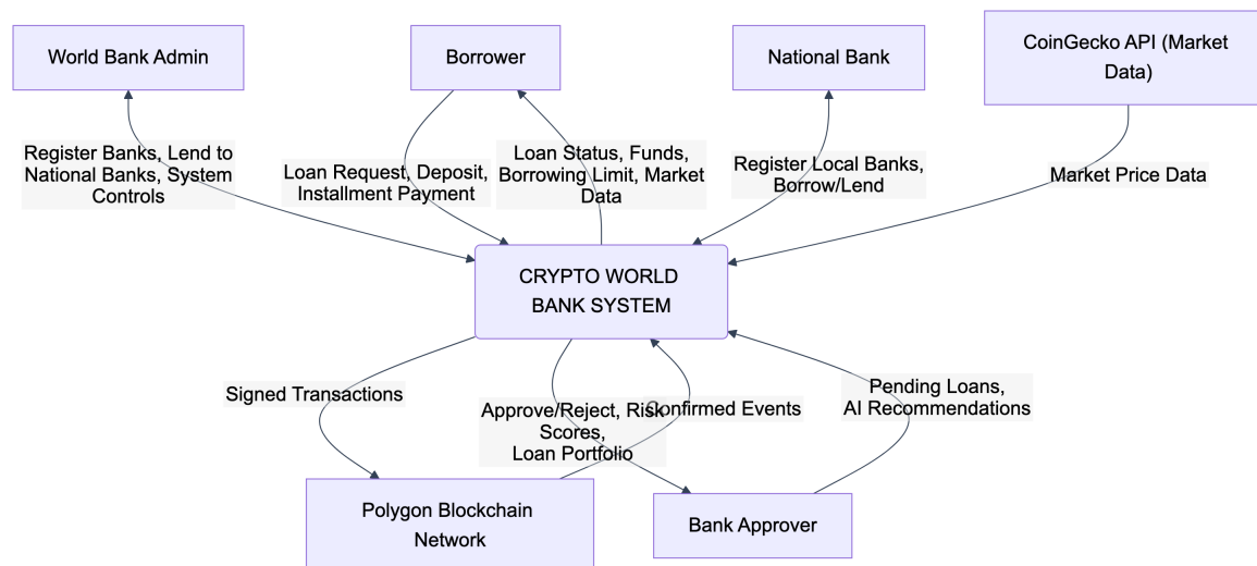
Figure 3.18: Dataflow Diagram (Context Diagram Level - 0)
