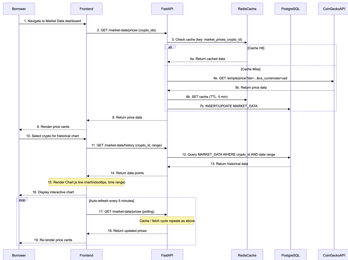
Figure 3.28: Sequence Diagram 7 Market Data Retrieval
